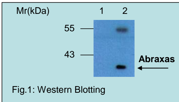
Fig. 1 : Western Blotting analysis of recombinant protein Abraxas produced in HEK293 transfected cells. SDS-PAGE Electrophoresis (Reducing conditions). Immunostaining with rabbit polyclonal antibody to Abraxas ; dilution 10 µg/ml (1, 2). Detection with goat anti-rabbit / HRP secondary antibody. Lane 1: HEK 239 non-transfected bacterial culture (cell lysate) - negative controls. Lane 2: HEK 239 transfected bacterial culture (cell lysate).
