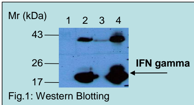
Fig. 1. Western Blotting analysis of recombinant protein h-IFN gamma produced in Escherichia coli BL21 ( \lambda .DE3) transfected bacterial culture. SDS-PAGE Electrophoresis (Reducing conditions). Rabbit was immunized with synthetic C-terminal peptide derived from IFN gamma. Immunostaining with rabbit polyclonal antibody to h-IFN gamma ; dilution 1 \mu g/ml (1, 2) non purified serum (3, 4). Detection with goat anti-rabbit / HRP secondary antibody. Lane 1, 3: Escherichia coli non-transfected bacterial culture (cell lysate) - negative controls. Lane 2, 4: Escherichia coli transfected bacterial culture (cell lysate).
