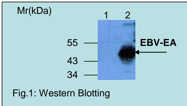
Fig. 1. Western Blotting analysis of recombinant protein EBV-EA produced in Escherichia coli BL21 ( \lambda DE3) transfected bacterial culture. SDS-PAGE Electrophoresis (Reducing conditions). Immunostaining with rabbit polyclonal antibody to EBV-EA ; dilution (1, 2) 0,1 \mu g/ml. Detection with goat anti-rabbit / HRP secondary antibody. Lane 1: Escherichia coli non-transfected bacterial culture (cell lysate) - negative controls. Lane 2: Escherichia coli transfected bacterial culture (cell lysate).
