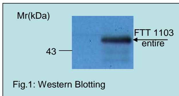
Fig. 1. Western Blotting analysis of recombinant protein FTT1103 entire produced in Escherichia coli BL21 ( \lambda .DE3) transfected bacterial culture. SDS-PAGE Electrophoresis (Reducing conditions). Immunostaining with rabbit polyclonal antibody to FTT1103 entire ; dilution (1, 2) 0,2 \mu g/ml. Detection with goat anti-rabbit / HRP secondary antibody. Lane 1: Escherichia coli non-transfected bacterial culture (cell lysate) - negative controls. Lane 2: Escherichia coli transfected bacterial culture (cell lysate).
