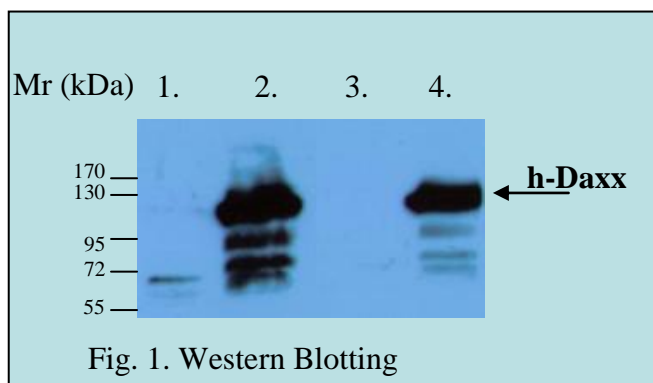
Fig. 1. Western Blotting analysis of recombinant protein h-Daxx produced in HEK293 transfected cells. SDS-PAGE Electrophoresis (Reducing conditions). Immunostaining with rabbit polyclonal antibody to h-Daxx ; dilution 0,5 µg/ml (1, 2) non purified serum (3, 4). Detection with goat anti-rabbit / HRP secondary antibody. Lane 1, 3: HEK 239 non transfected cells (cell lysate) - negative controls. Lane 2, 4: HEK 239 transfected cells (cell lysate).
