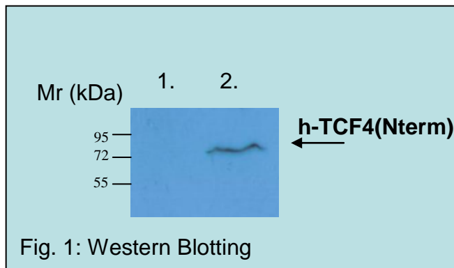
Fig. 1. Western Blotting analysis of recombinant protein h-TCF4 produced in HEK293 transfected cells. SDS-PAGE Electrophoresis (Reducing conditions). Immunostaining with rabbit polyclonal antibody to h-TCF4 (Nterm) ; dilution (1,2) 1 µg/ml. Detection with goat anti-rabbit / HRP secondary antibody. Lane 1: HEK 239 non transfected cells (cell lysate) - negative controls. Lane 2: HEK 239 transfected cells (cell lysate).
